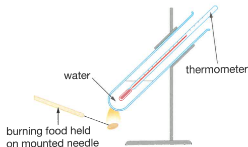
▲ Figure 4.13 Measuring the energy content of a food sample
