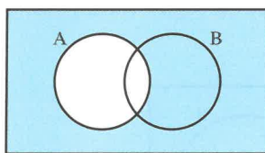
The complement A' of set A
