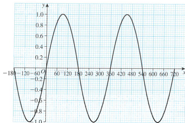
Graph of y = \sin x from -180^\circ to 720^\circ
