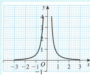
A typical reciprocal curve y = \frac{1}{x^2}
