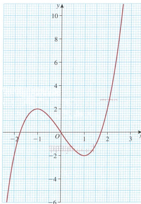
Graph of y = x^3 - 3x
