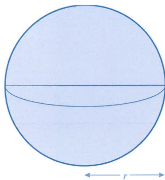
Surface area of a sphere A = 4\pi r^2
