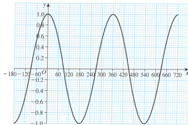
Graph of y = \cos x from -180^\circ to 720^\circ
