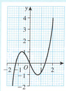
A typical cubic curve y = x^3 - 2x
