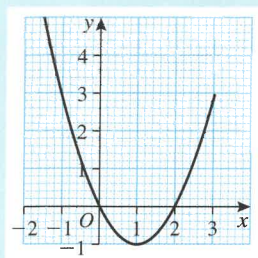
A typical quadratic curve y = x^2 - 2x
