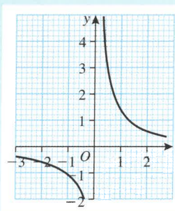
A typical reciprocal curve y = \frac{1}{x}
