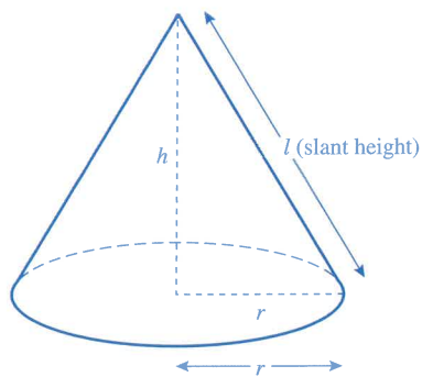
(Curved) Surface area of a cone A = \pi r l
