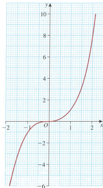
Graph of y = x^3
