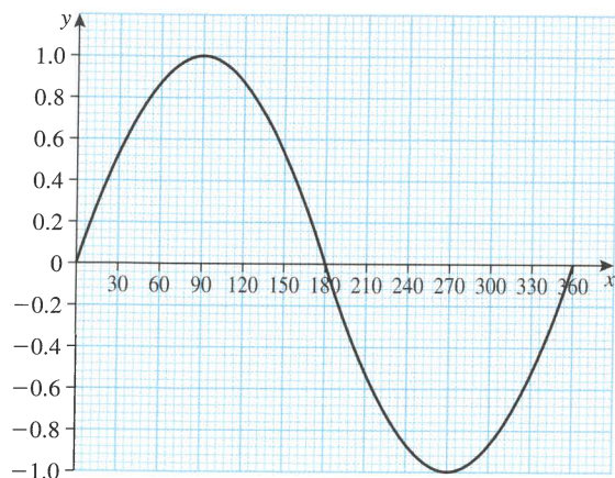
Graph of y = \sin x from 0^\circ to 360^\circ
